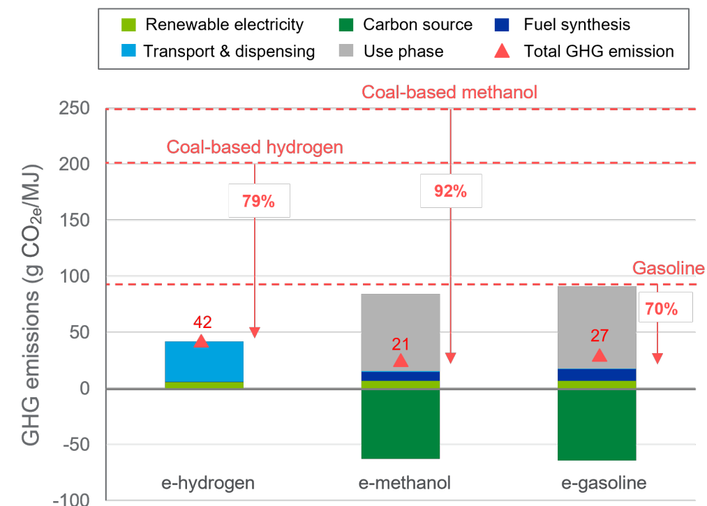
Figure 5 | GHG emissions of e-hydrogen, e-methanol, and e-gasoline
